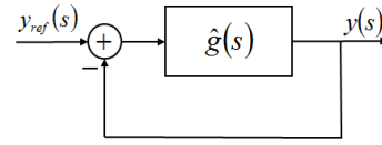
Fig. 1. Simple feedback.
